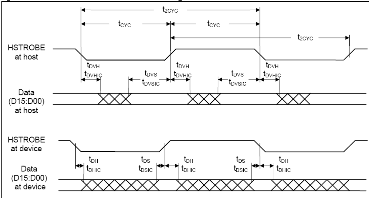
Figure 16: Sustained Ultra DMA Data-Out Burst Timing
