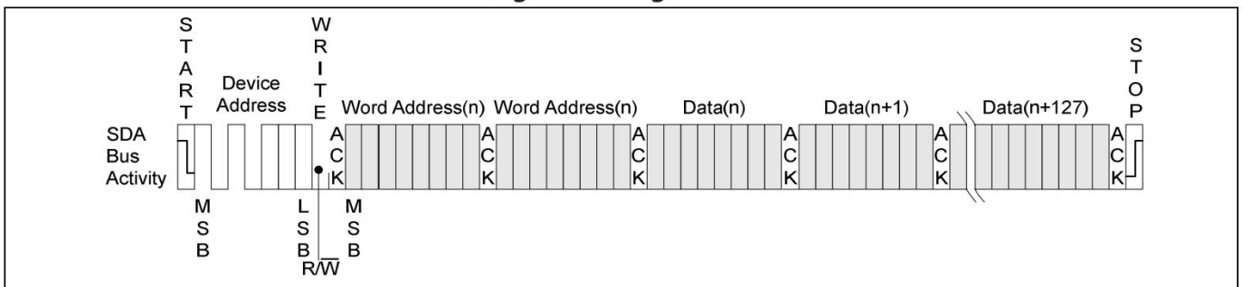
Figure 1-7. Page Write
