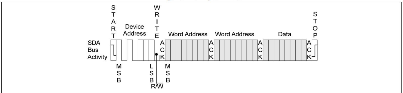
Figure 1-6. Byte Write
