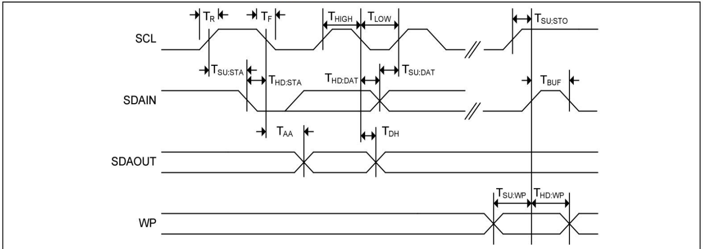
Figure 1-11. Bus Timing
