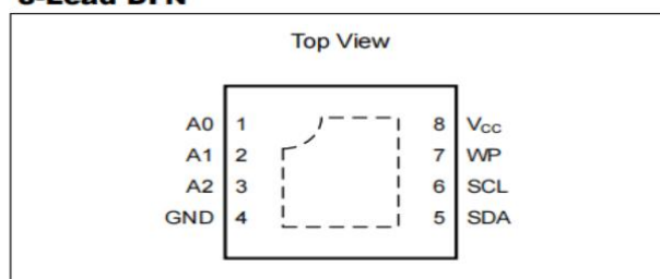
8-Lead DFN
