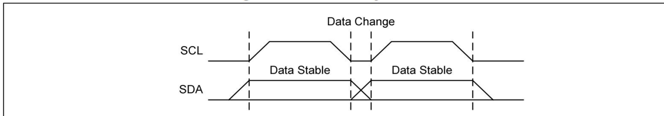
Figure 1-4. Data Validity Protocol
