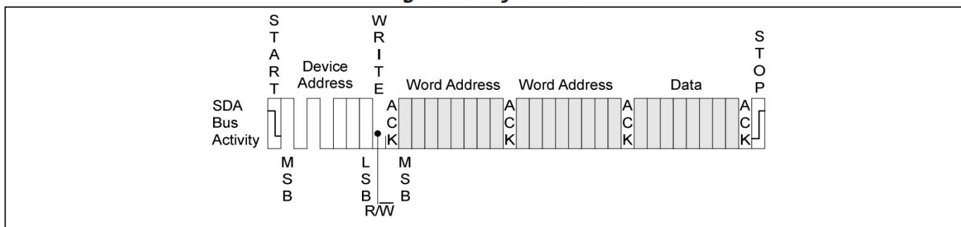
Figure 1-6. Byte Write
