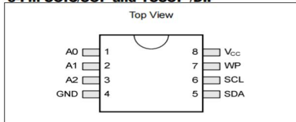
8-Pin SOIC/SOP and TSSOP /DIP
