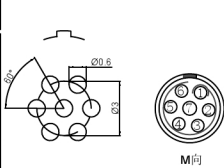
Pcb plate opening size (PCB板开孔尺寸)
