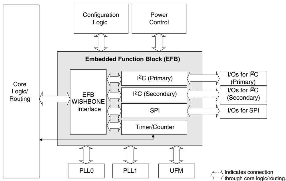
Figure 2-20. Embedded Function Block Interface
