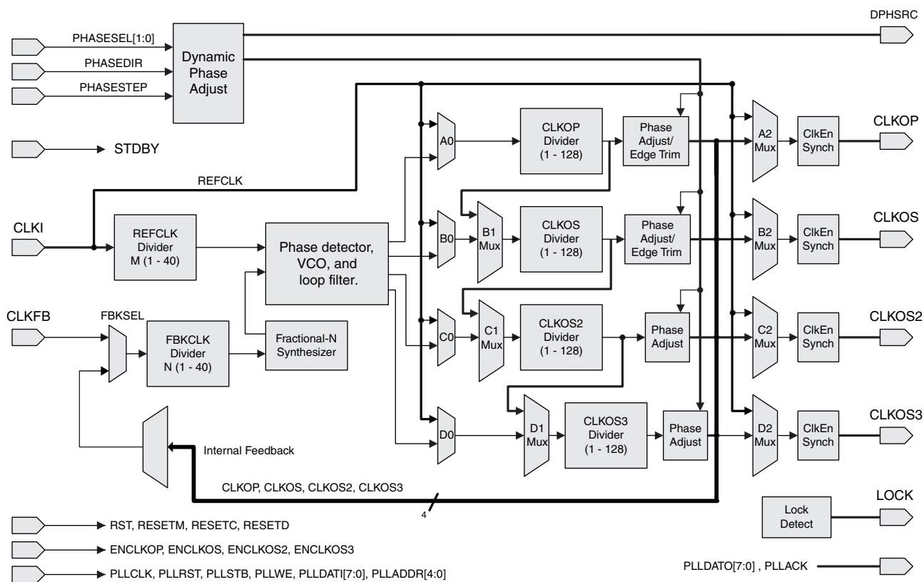
Figure 2-7. PLL Diagram
