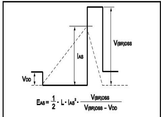
Fig.12 Avalanche Waveform
