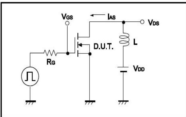
Fig.11 Avalanche Measurement Circuit
