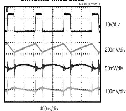
SWITCHING WAVEFORMS
