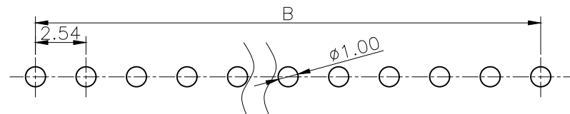
Recommended P.C.B Layout
