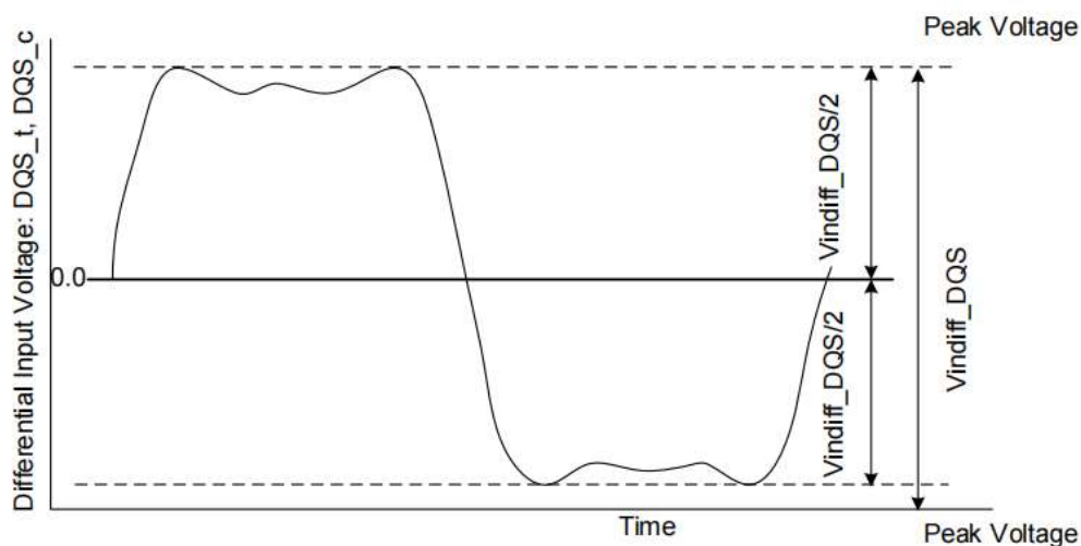
Figure 5-9 DQS Differential Input Voltage
