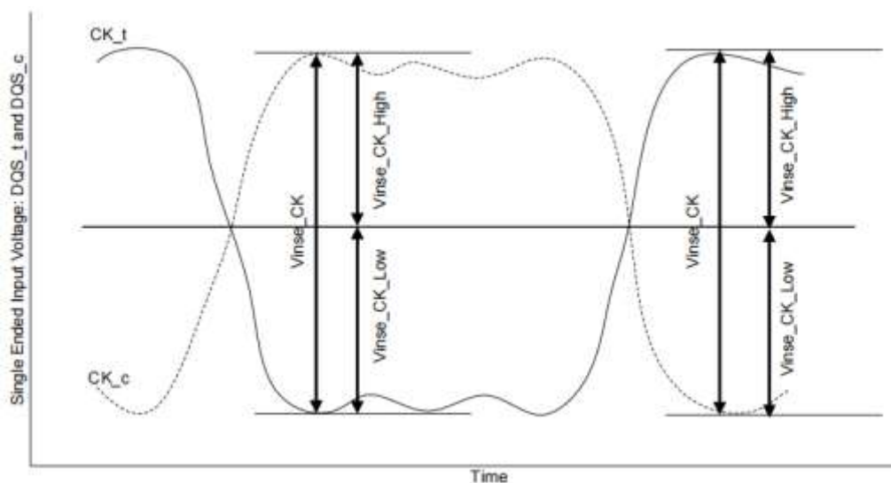
Figure 5-6 Clock Single-Ended Input Voltage
