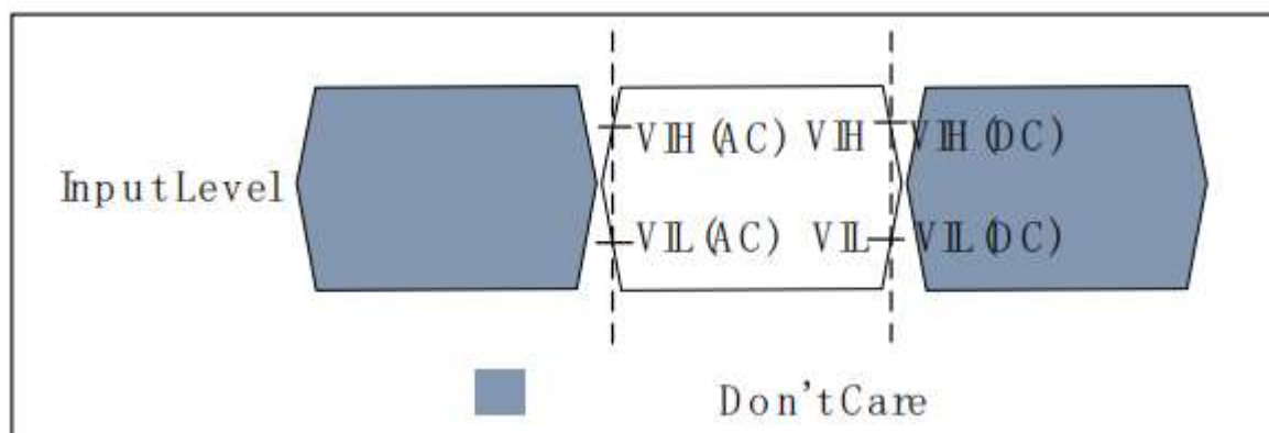
Figure 5-1 Input AC Timing Definition for CKE
