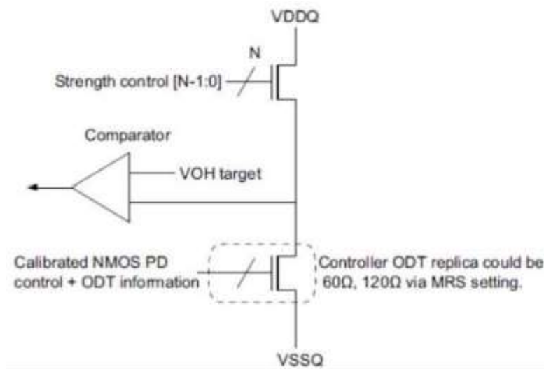
Figure 5-18 Pull-up Calibration
