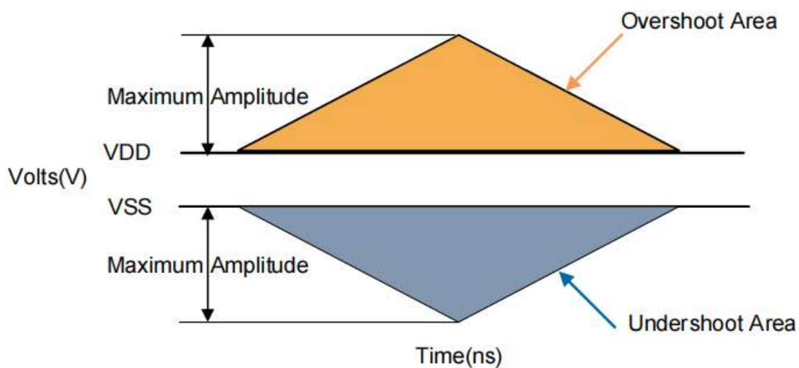
Figure 5-3 AC Overshoot and Undershoot Definition for Address and Control Pins
