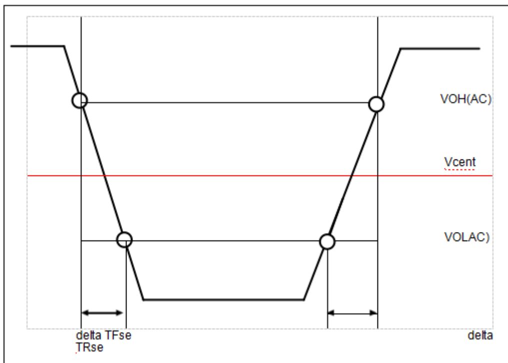
Figure 4-1 Single Ended Output Slew Rate Definition
