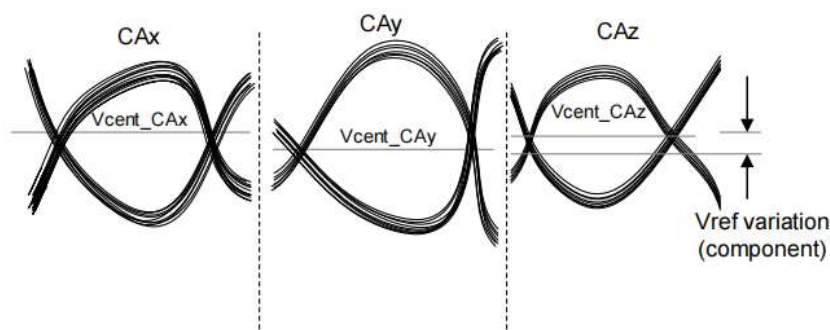
Figure 8-2 Across Pin VREFCA Voltage Variation
