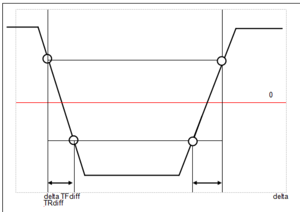
Figure 4-2 Differential Output Slew Rate Definition
