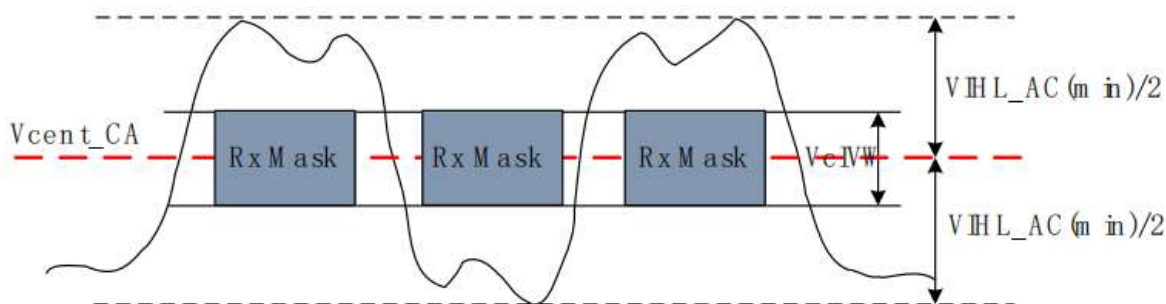
Figure 8-5 CA VIH_L_AC Definition (for Each Input Pulse)
