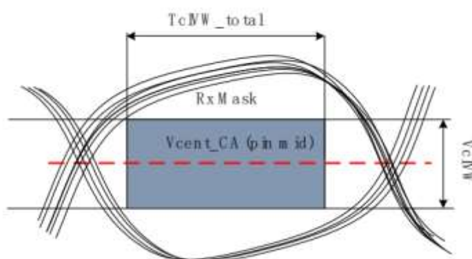
Figure 8-1 CA Receiver (Rx) Mask
