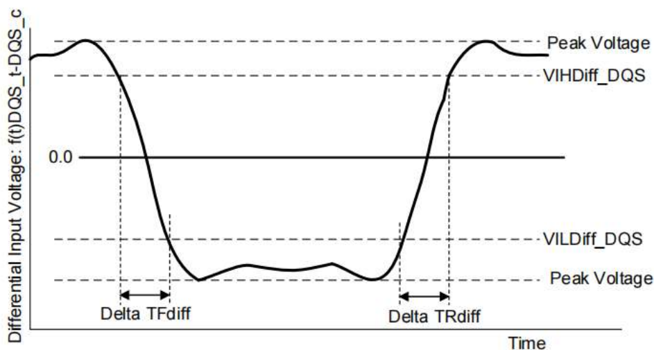
Figure 5-12 Differential Input Slew Rate Definition for DQS t , DQS c
