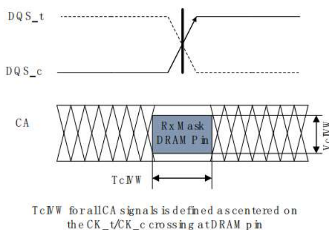
Figure 8-3 CA Timings at the DRAM Pins
