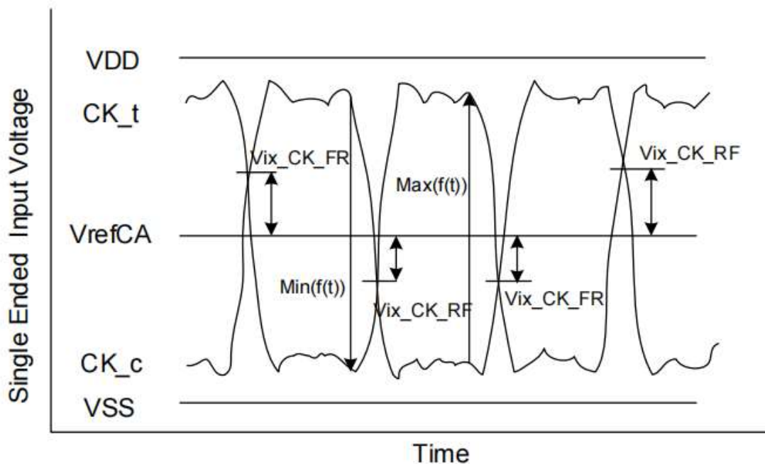
Figure 5-8 Vix Definition (Clock)
