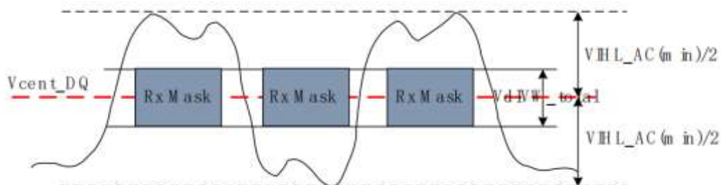
Figure 8-12 DQ VIH_L_AC definition (for Each Input Pulse)
