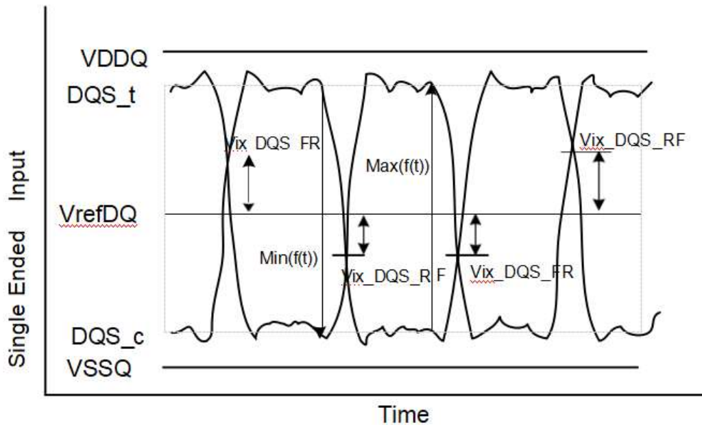
Figure 5-13 Vix Definition (DQS)
