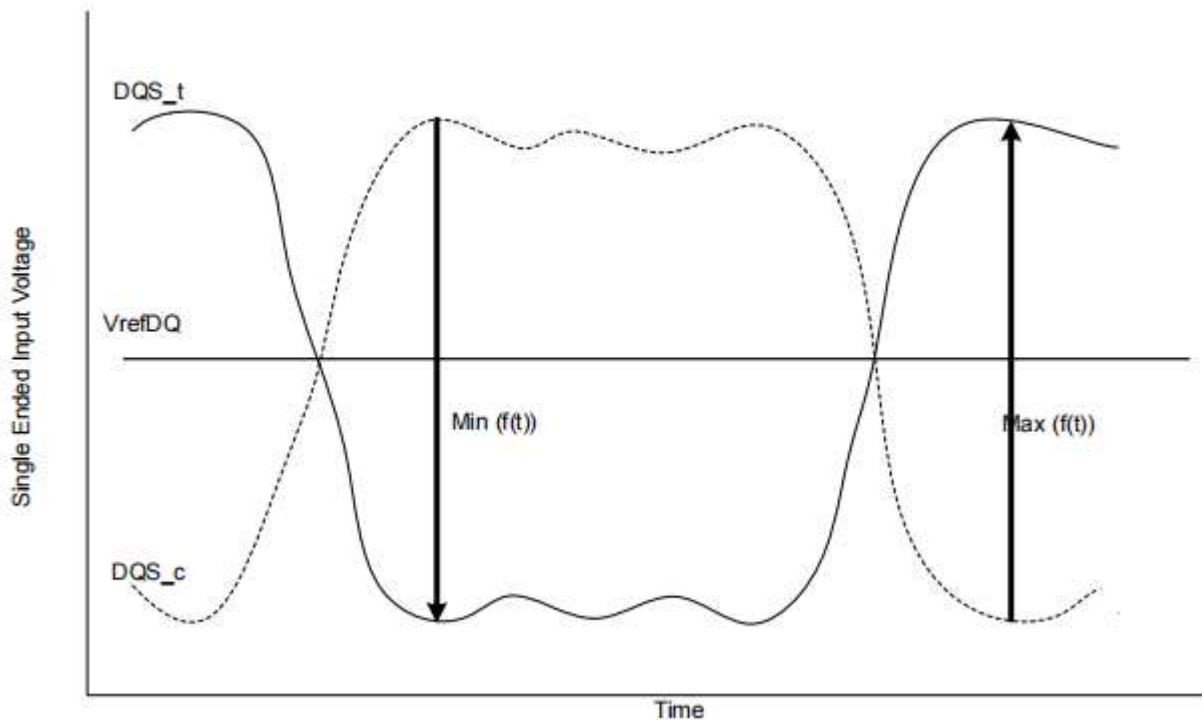
Figure 5-10 Definition of Differential DQS Peak Voltage
