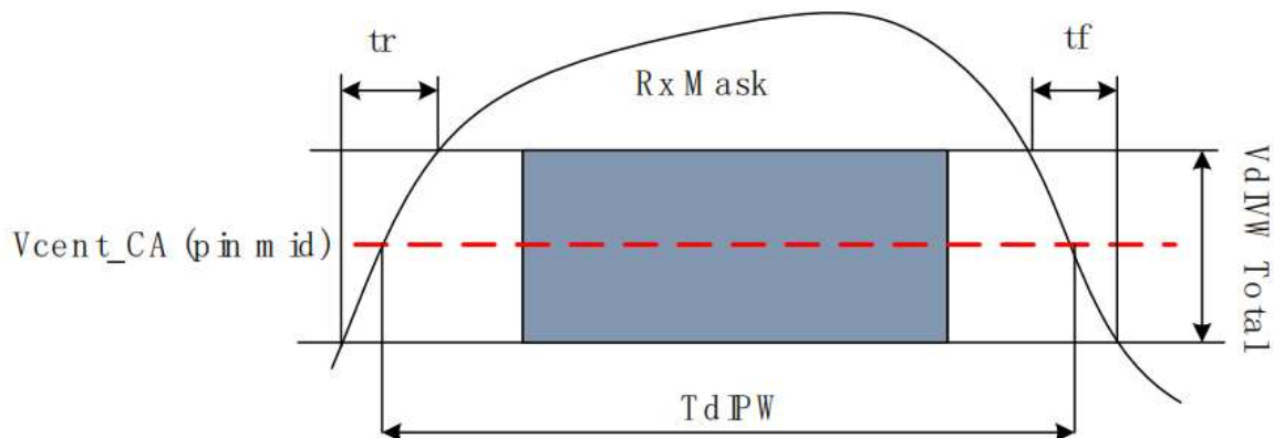
Figure 8-11 TdIPW and SRIN_dIVW Definition (for Each Input Pulse)
