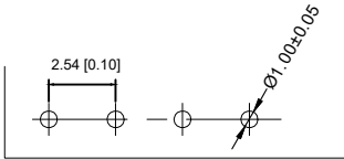
Recommmand PCB Layout
