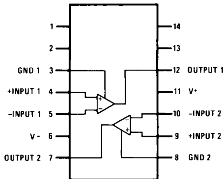
Dual-In-Line Package
