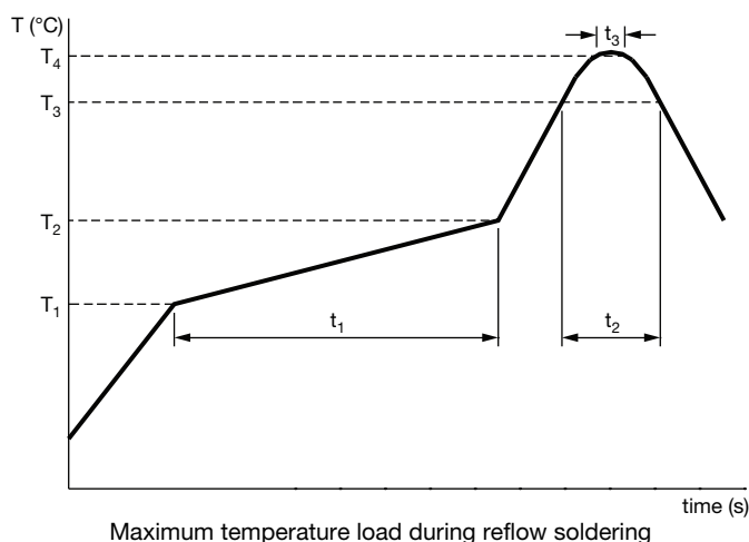
Maximum temperature load during reflow soldering
