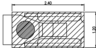
P.C.B LAYOUT TOLERANCE:±0.05
