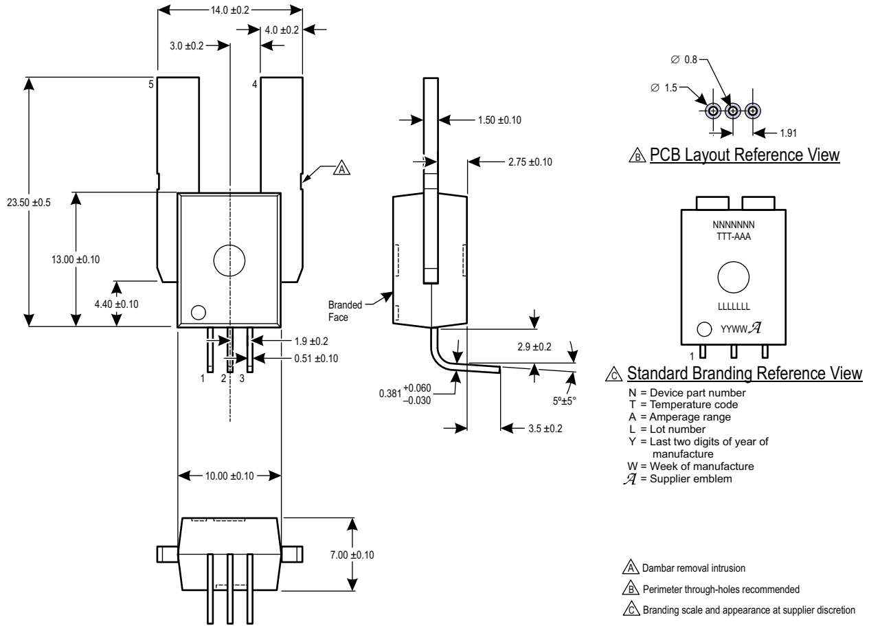
Figure 10: Package CB, 5-Pin, Leadform PSF
