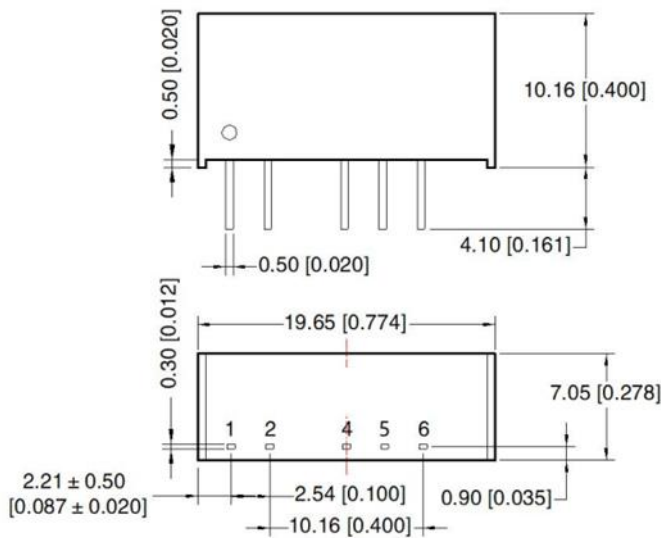
Figure 7: Overall dimensions
