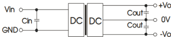
Figure 1: Application circuit
