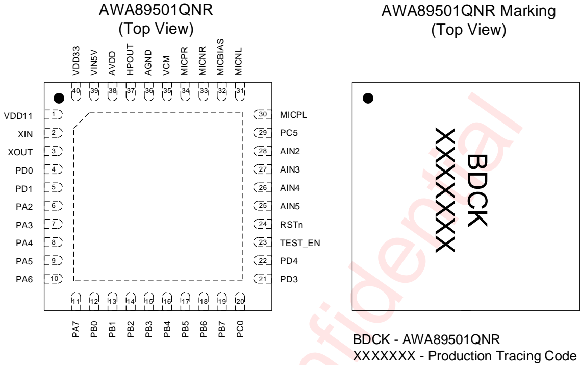
Figure 1 AWA89501 pin diagram top view and device marking
