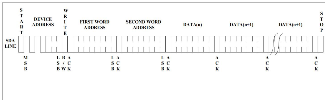
Figure 7. Page Write
