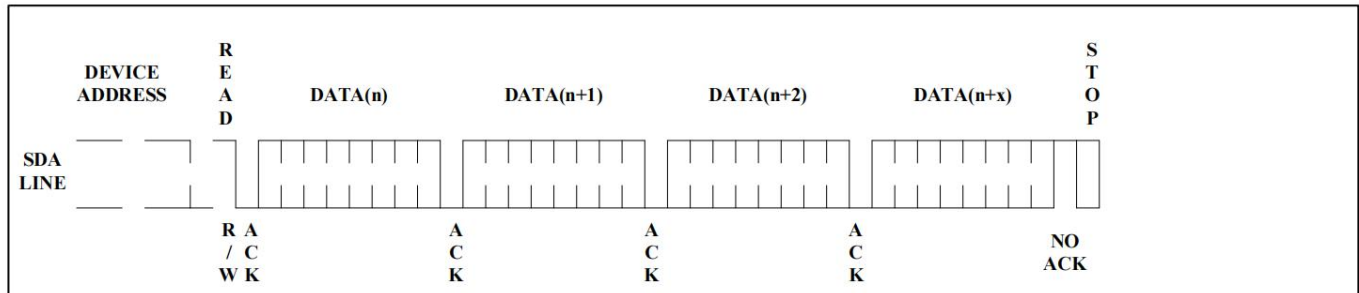
Figure 10. Sequential Read
