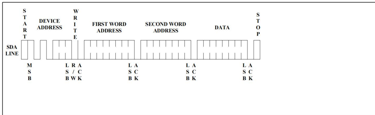
Figure 6. Byte Write
