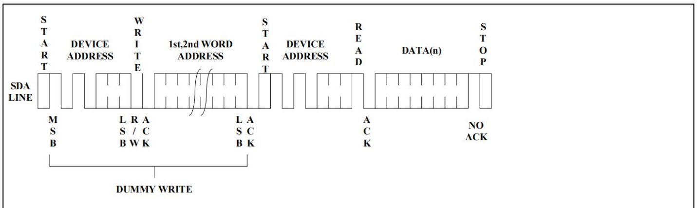
Figure 9. Random Read
