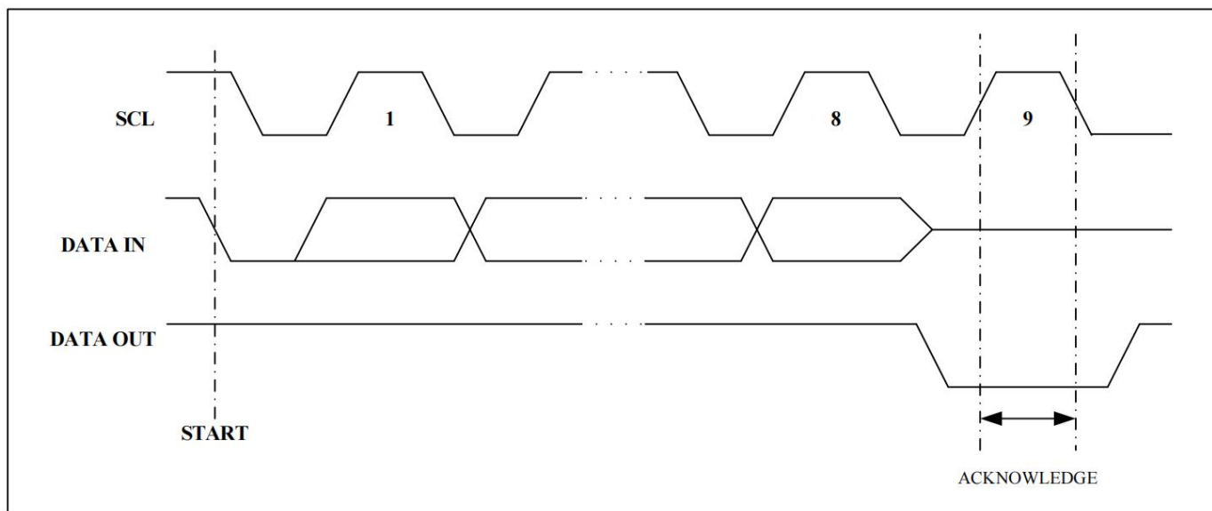
Figure 4. Output Acknowledge
