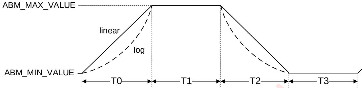
Figure 10 autonomous breathing mode
