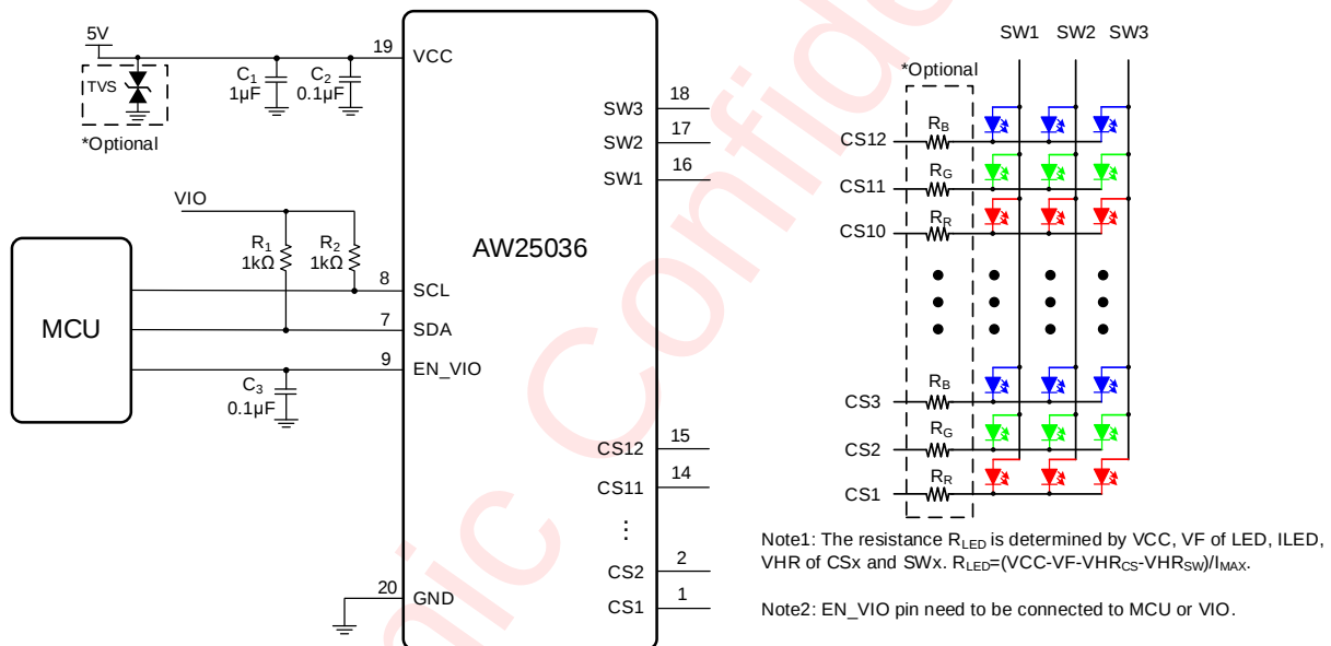
Figure 22 Application Circuit
