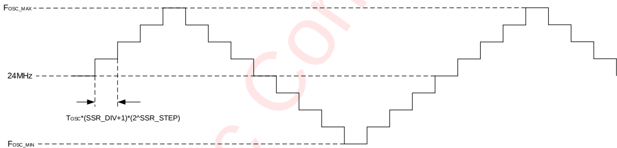
Figure 12 spread spectrum
