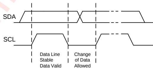
Figure 17 Data Validation Diagram
