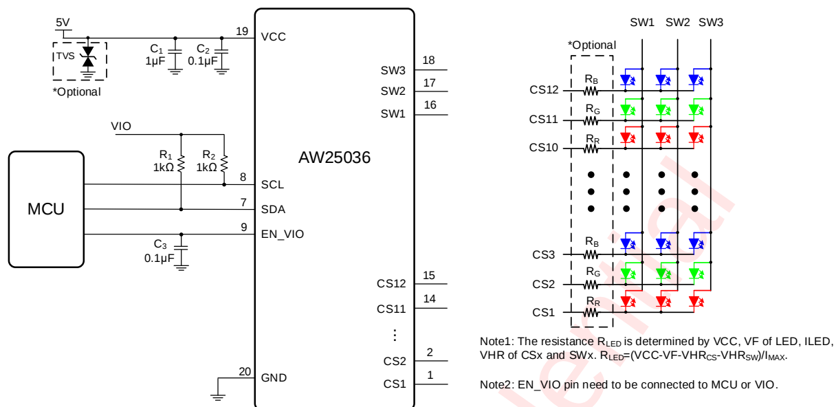
Figure 1 AW25036 Application Circuit
