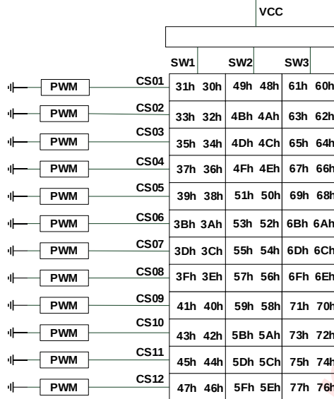
Figure 9 12-bit PWM data storage addresses
