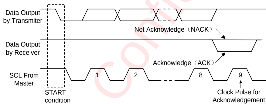
Figure 19 I²C ACK Timing
