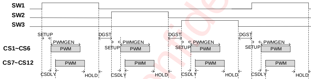
Figure 7 overall timing sequence
