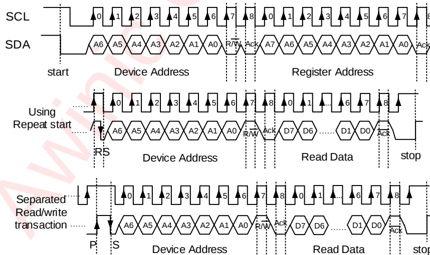
Figure 21 I²C Read Byte Cycle
