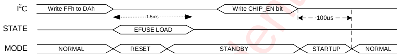
Figure 16 Soft-Reset process in I 2 C MODE
