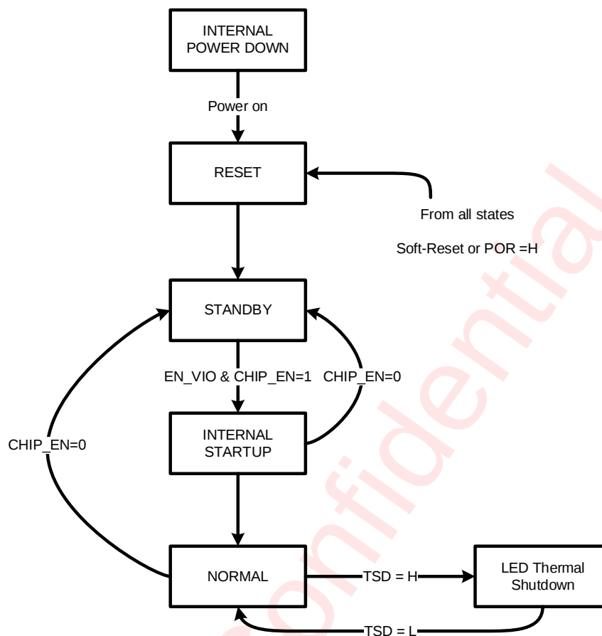
Figure 15 operating mode transition
