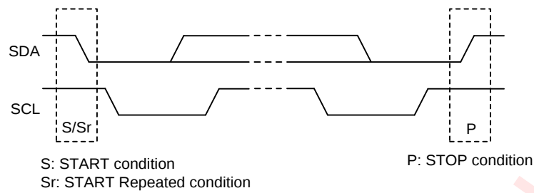
Figure 18 I²C Start/Stop Condition Timing
