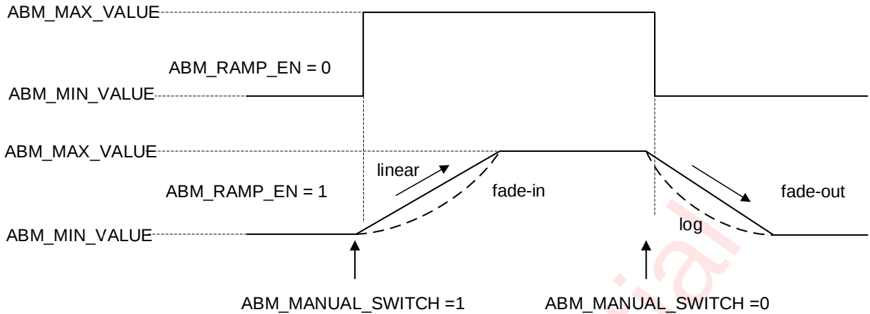
Figure 11 Manual switch mode
