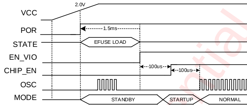
Figure 5 Startup Timing
