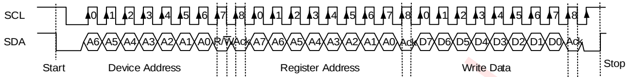
Figure 20 I²C Write Byte Cycle
