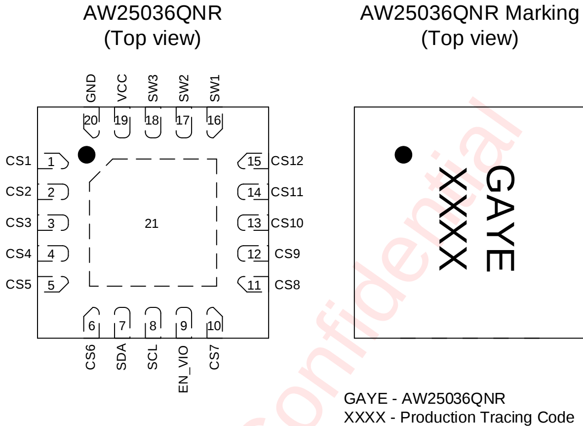
Figure 2 Pin Configuration and Top Marking
