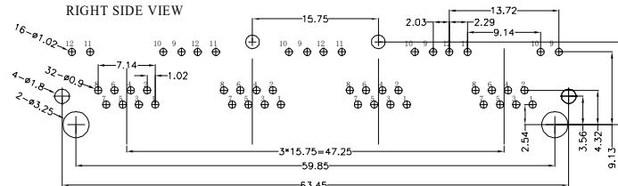
RECOMMENDED PCB LAYOUT VIEWED FROM COMPONENT SIDE
