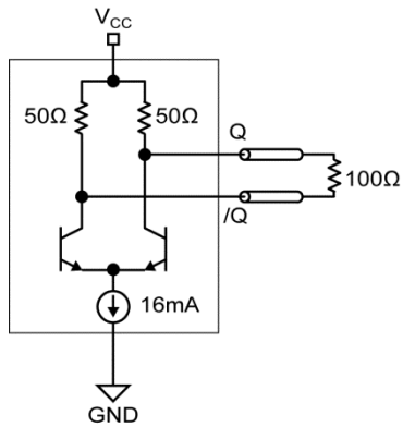
Figure 10. CML DC-Coupled
