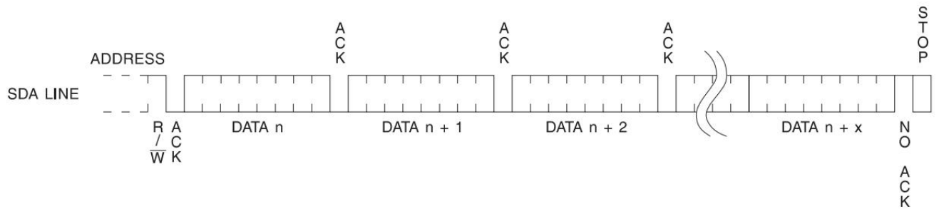
Figure 4. Sequential Read
