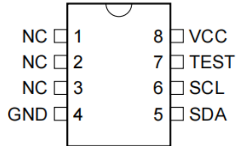
8-Pin PDIP
