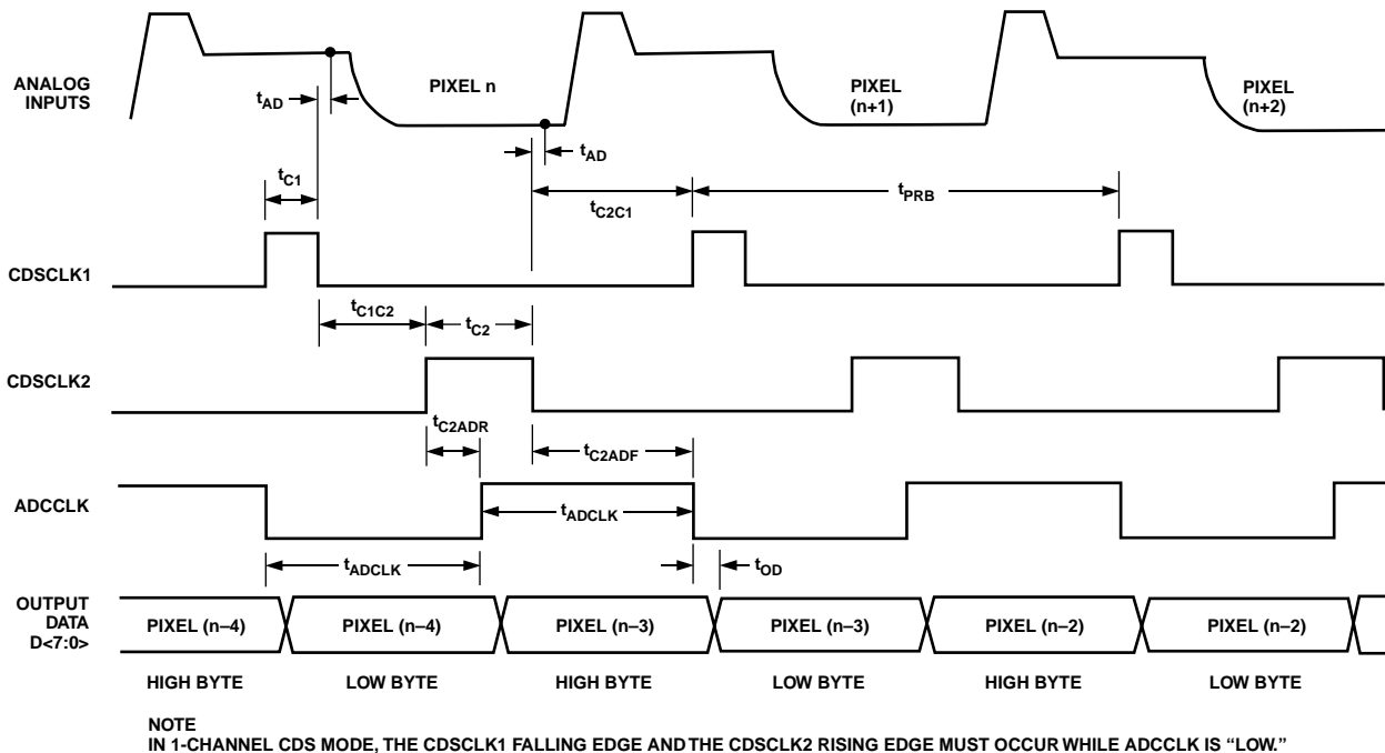
Figure 2. 1-Channel CDS Mode Timing
