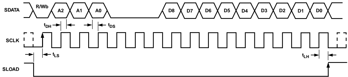
Figure 9. Serial Write Operation Timing
