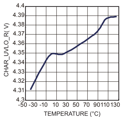
VUVLO_rising vs. Temperature
