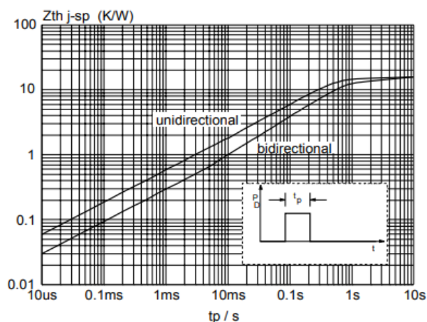
Fig.11. Transient thermal impedance Z_{th \text{ j-sp}} , versus pulse width t_p .
