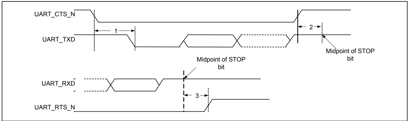
Figure 13. UART Timing
