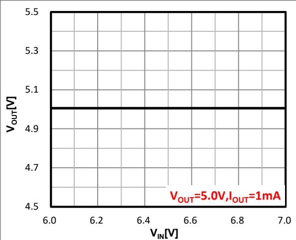
Figure 18. Line Regulation
