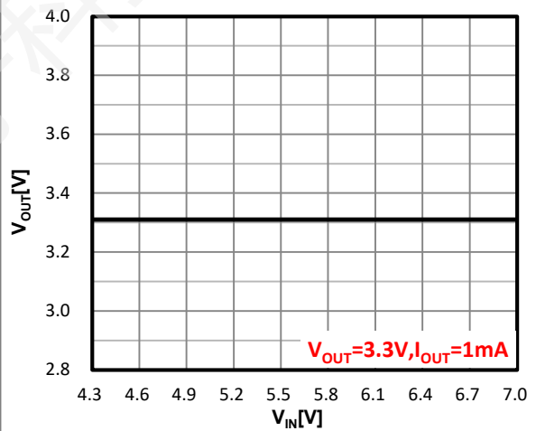
Figure 16. Line Regulation
