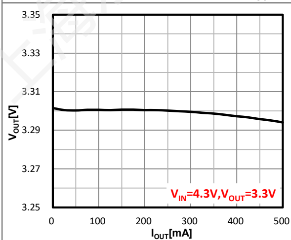
Figure 23. Load Regulation
