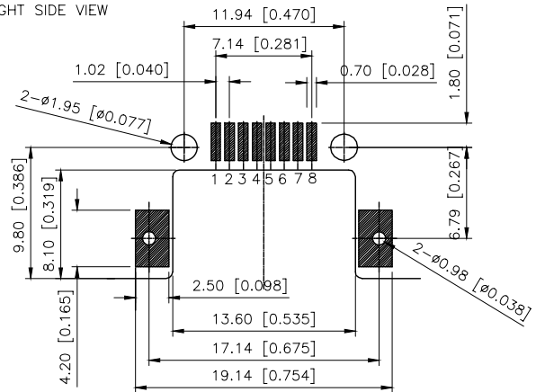
RECOMMENDED PCB LAYOUT VIEWED FROM COMPONENT SIDE
