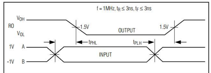
Figure 10. Receiver Propagation Delays
