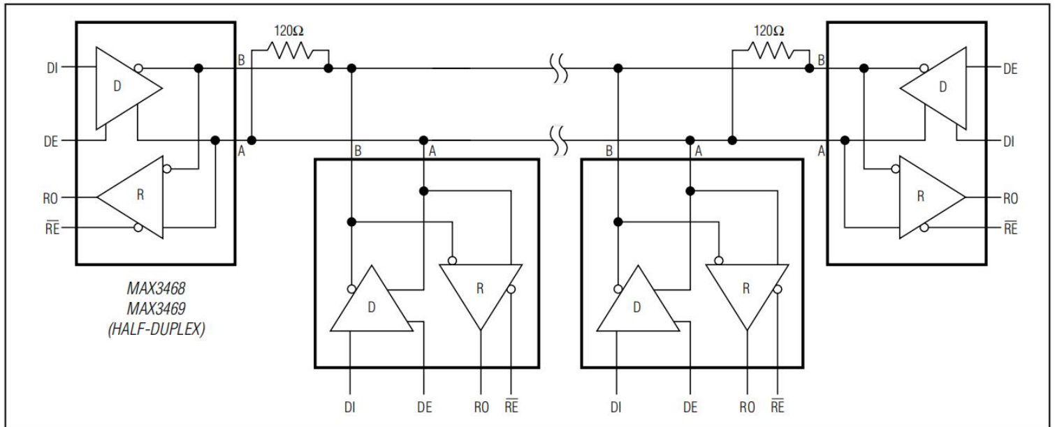
Figure 13. Typical Half-Duplex RS-485 Network
