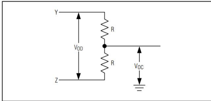
Figure 5. Driver DC Test Load
