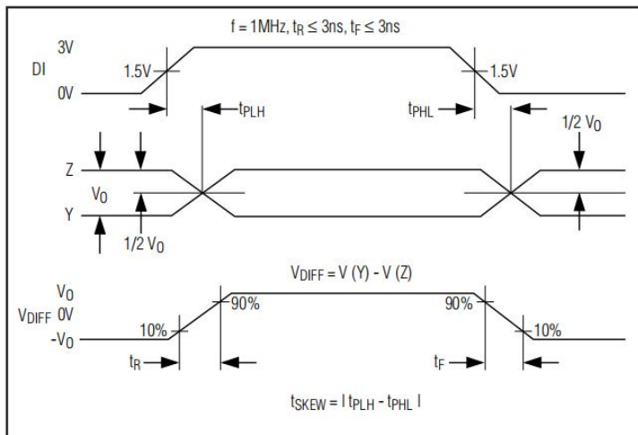
Figure 7. Driver Propagation Delays
