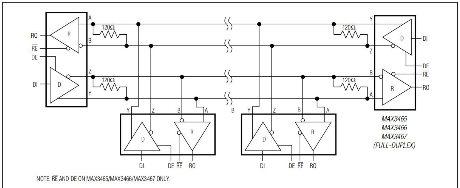
Figure 14. Typical Full-Duplex RS-485 Network
