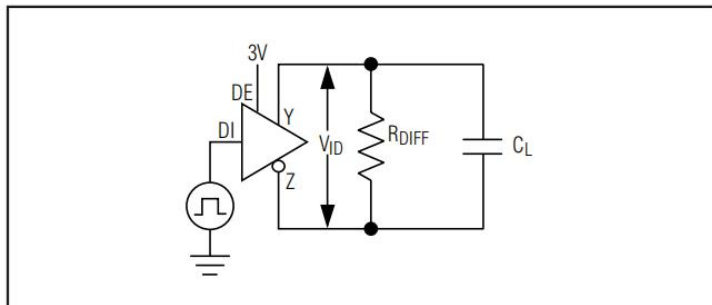
Figure 6. Driver Timing Test Circuit
