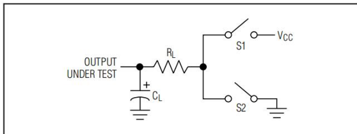
Figure 8. Enable/Disable Timing Test Load
