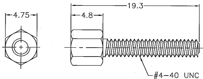
Screw: 2pcs
