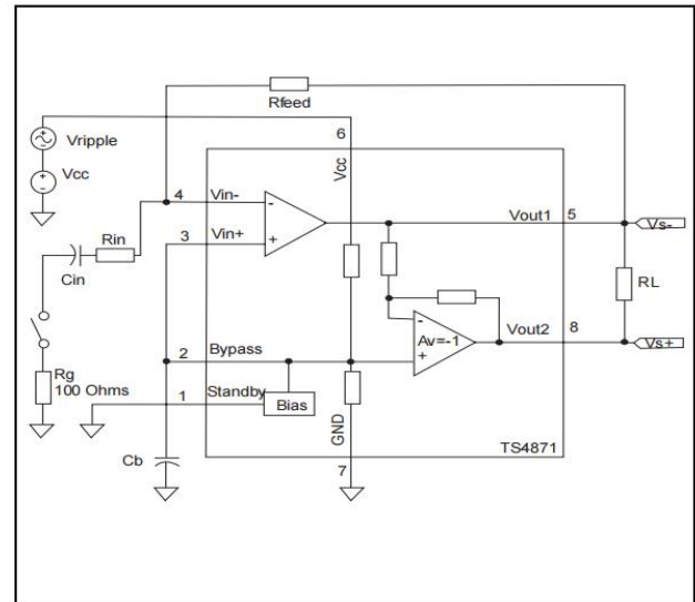
Fig. 86 : PSRR measurement schematic
