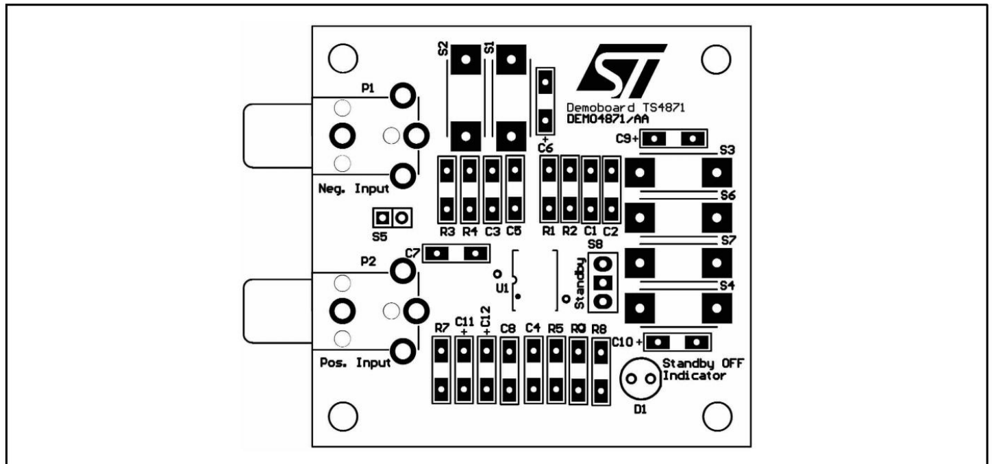
Fig. 82 : SO8 & MiniSO8 Demoboard Components Side
