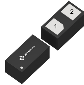
DFN0603-2L (DFN-2L(0.6x0.3))
