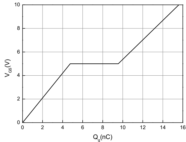
Figure 7. Typical Gate Charge ( I_{DS} = 4A , V_{DS} = 400V )
