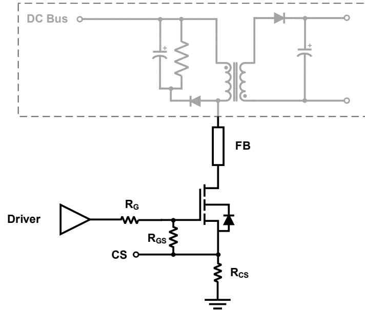
Figure 13. Simplified flyback schematic
