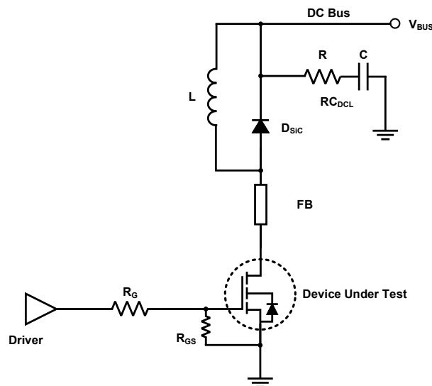
Figure 14. Switching test circuit for inductive load
