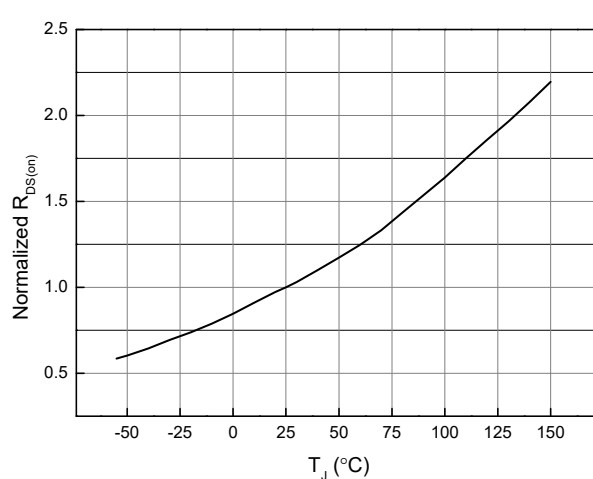
Figure 4. Normalized On-Resistance ( I_D = 4\text{A} , V_{GS} = 10\text{V} )
