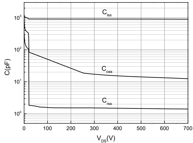
Figure 5. Typical Capacitance ( V_{GS} = 0V , f = 500kHz )
