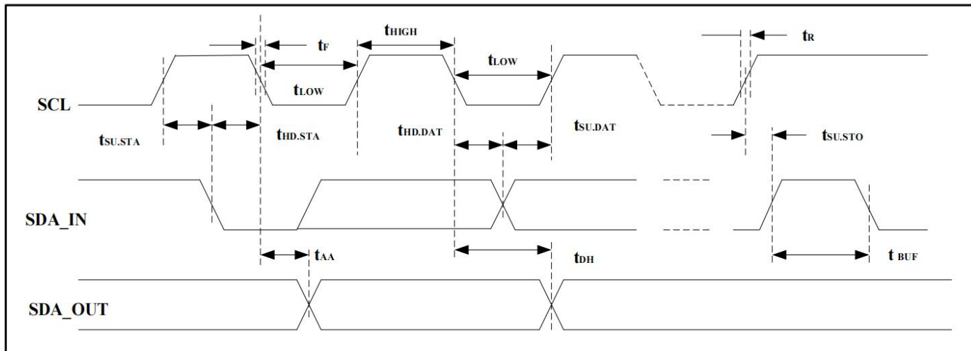
Figure 11. SCL: Serial Clock, SDA: Serial Data I/O
