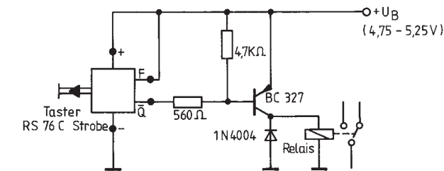
Driving of a PNP transistor
