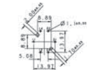
PCB hole pattern, component side
