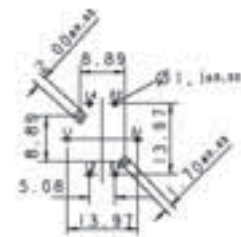
PCB hole pattern, component side
