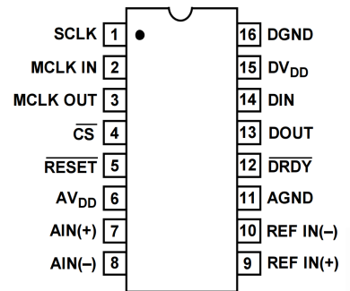
Pin Configuration
