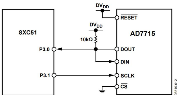
Figure 12. AD7715 to 8XC51 Interface
