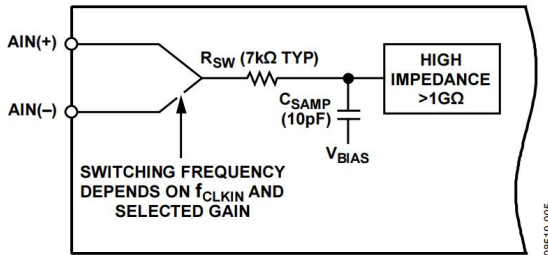
Figure 5. Unbuffered Analog Input Structure
