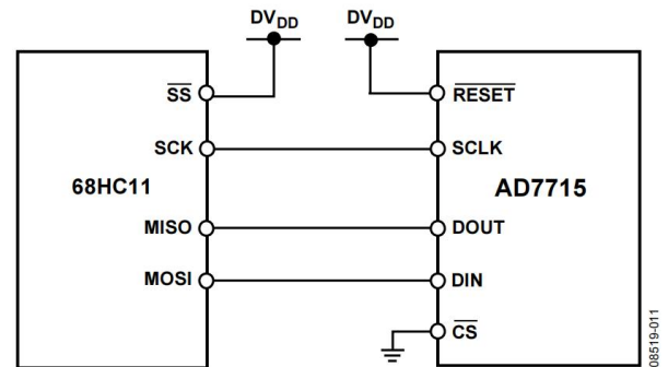
Figure 11. AD7715 to 68HC11 Interface
