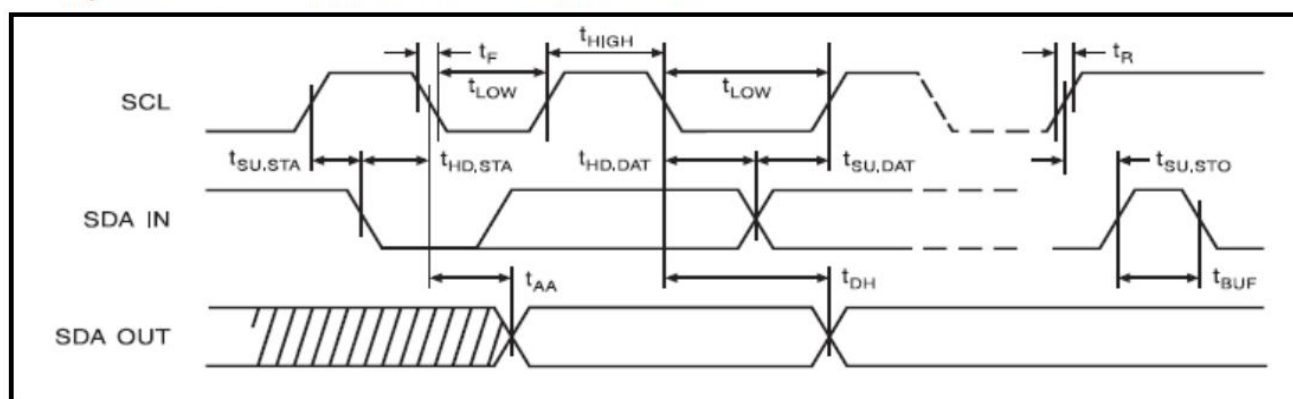
Figure 10. SCL: Serial Clock, SDA: Serial Data I/O
