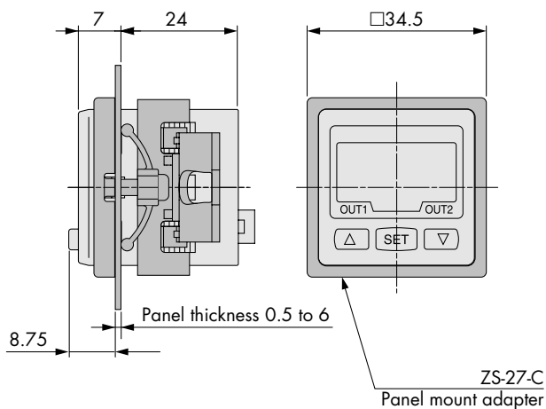
With panel mount adapter
