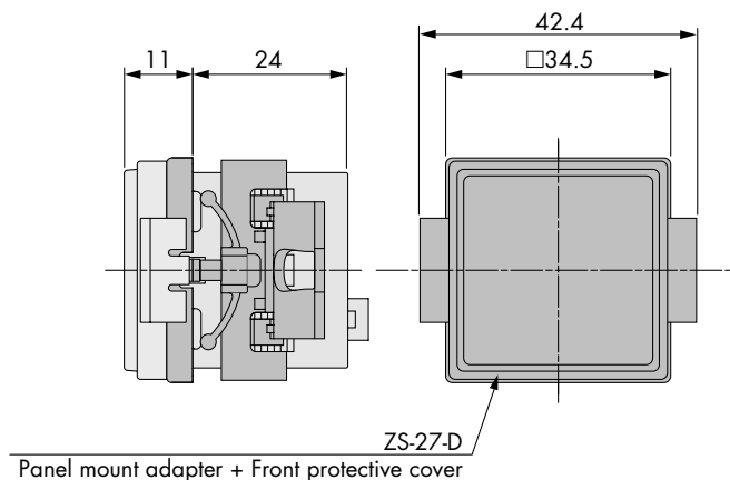
With panel mount adapter + Front protective cover
