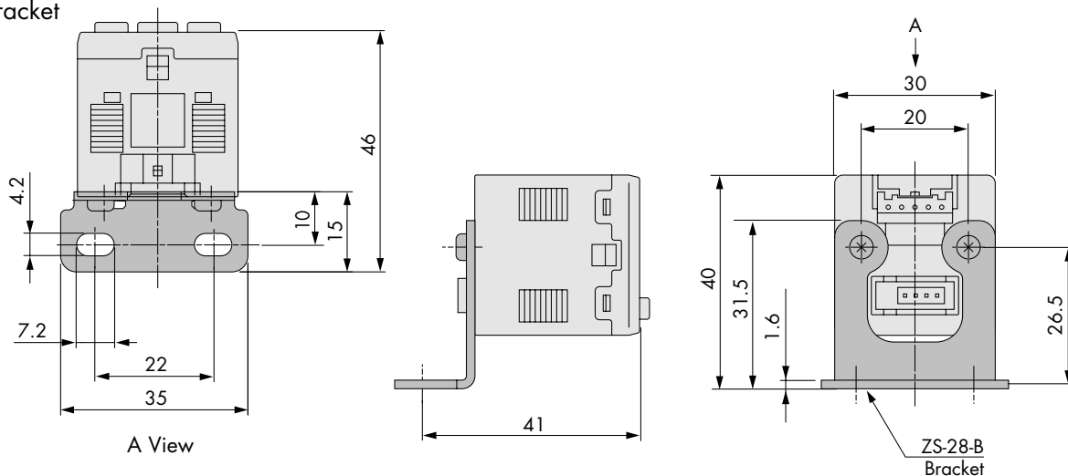
With panel mount adapter
