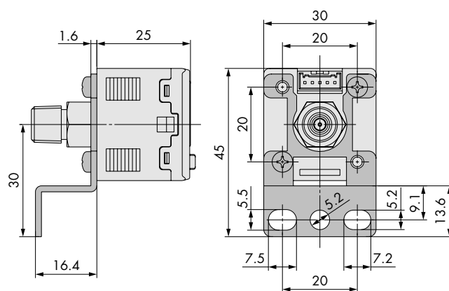
Bracket B
