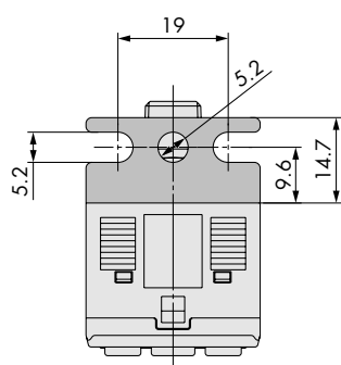
Bracket A
