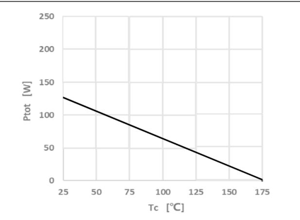
Figure 4. Power Dissipation
