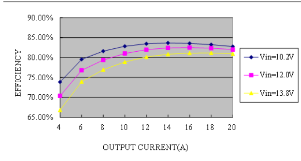
Figure 2. VID=0x62 ( V_o = 1.0V at no load) , PSI#=0
