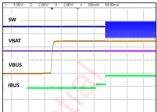
V_{BAT}=3.4V , OTG=0 Figure 13 Charge startup at VBUS plug-in
