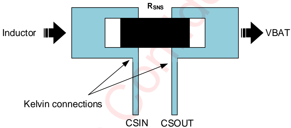
Figure 38 Sense Resistor PCB Layout
