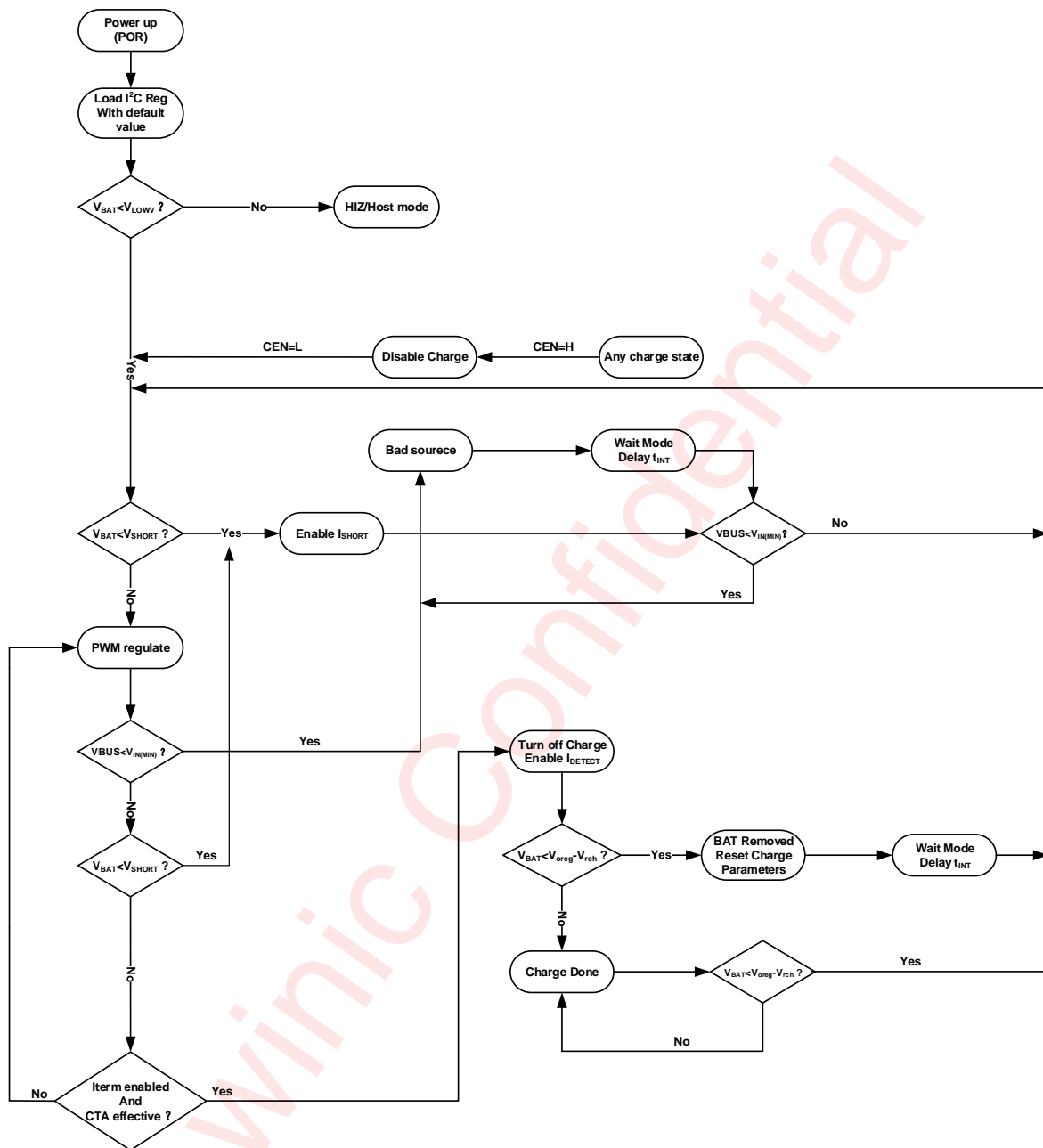
Figure 28 Charge Flow Chart of AW32257
