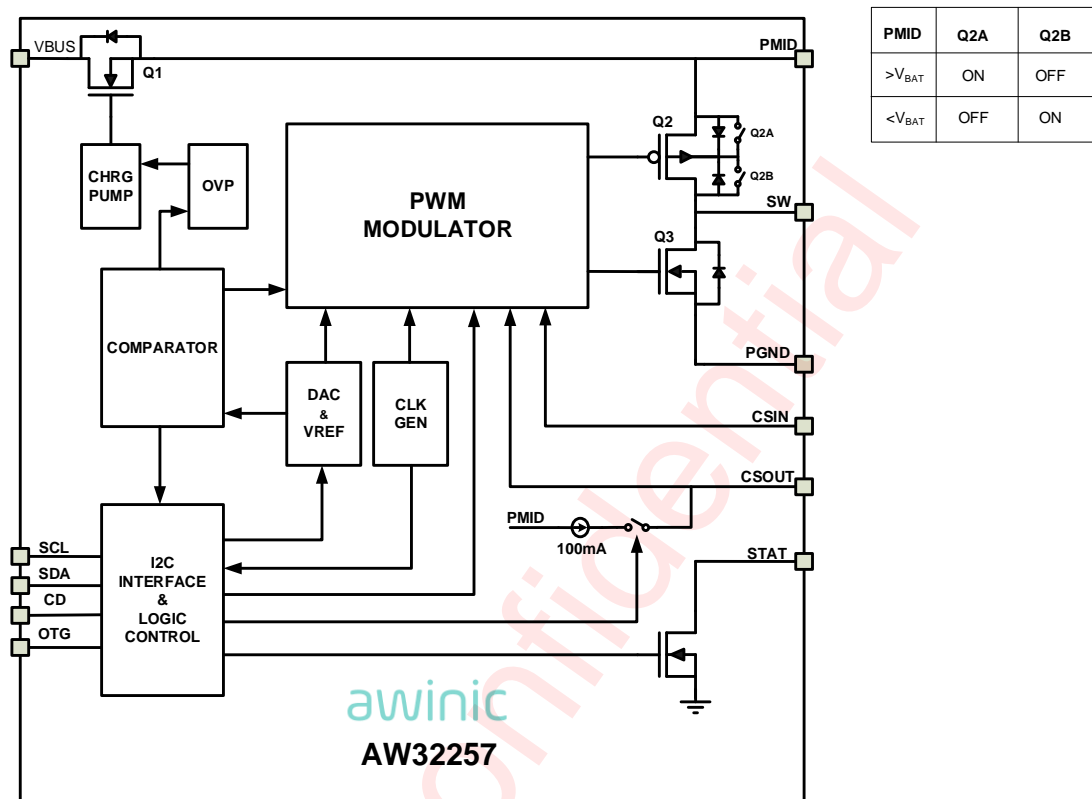
Figure 26 The AW32257 Function Block
