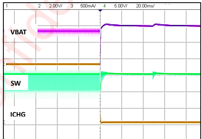
V_{BAT}=3.9V , I_{CHG}=1.86A , TE=1 Figure 15 Battery removal during charging
