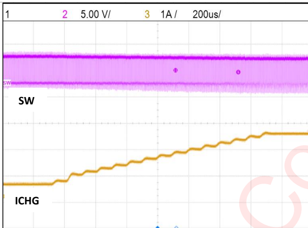
Figure 6 PWM charging waveform
