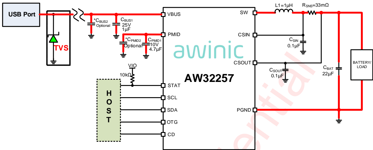
Figure 3 AW32257 Application Circuit
