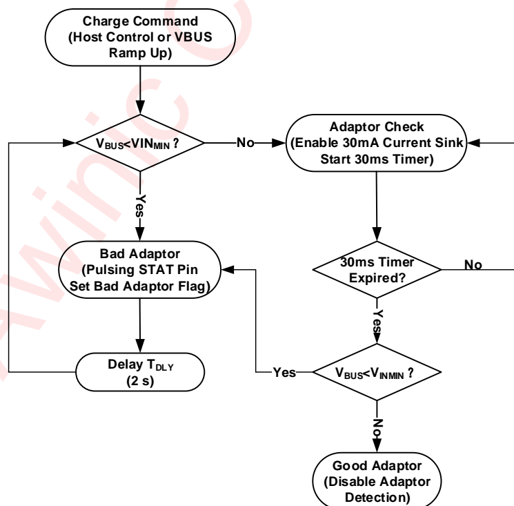
Figure 29 Bad Adaptor Detection Scheme Flow Chart
