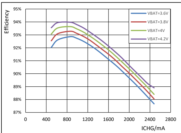
V_{BUS}=5V , DCR of Inductor is 23m\Omega Figure 12 Charge efficiency vs. VBAT
