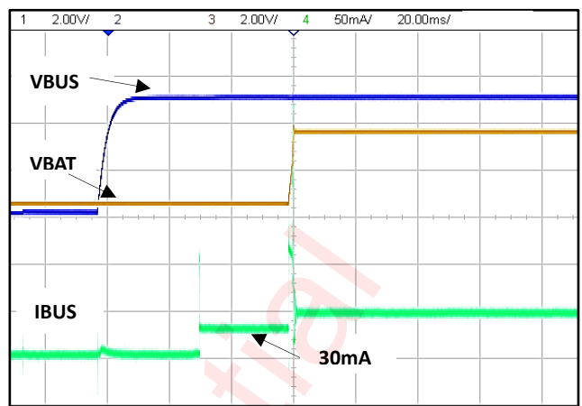
Figure 7 VBUS power up
