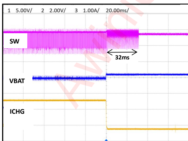
Figure 10 Charge termination detection
