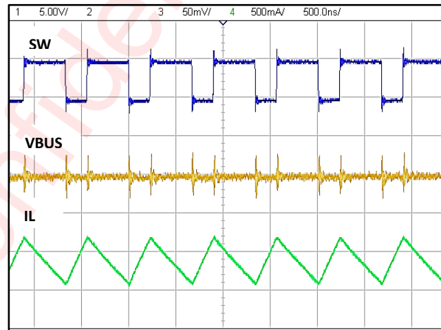
Figure 21 Boost PWM waveform
