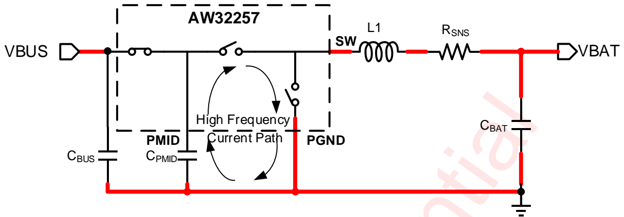
Figure 37 High Frequency Current Path
