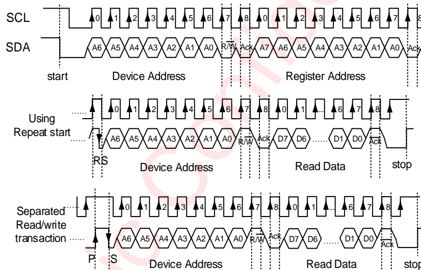
Figure 36 I 2 C Read Timing
