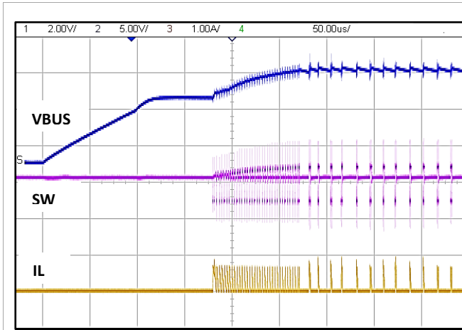
Boost start up with V_{BAT}=3.6V , I_{LOAD}=20mA , C_{BUS1}=10\mu F Figure 24 Boost startup
