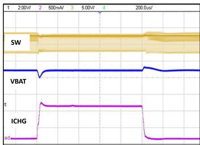
Figure 11 Load transient in download mode
