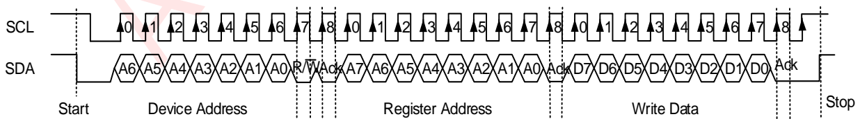
Figure 35 I 2 C Write Timing
