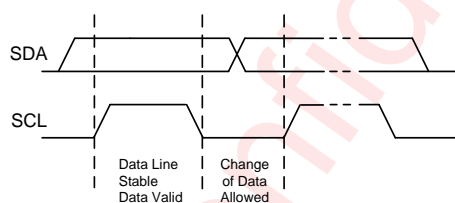
Figure 32 Data Validation Diagram
