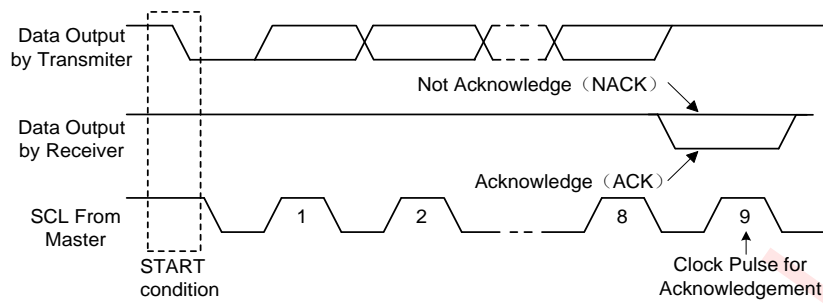
Figure 34 Acknowledgement Diagram
