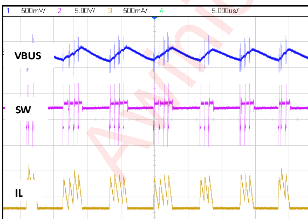
Figure 22 Boost BURST mode waveform
