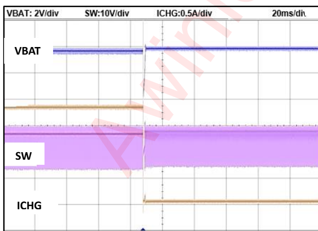
V_{BAT}=3.9V , I_{CHG}=1.86A , TE=0 Figure 16 Battery removal during charging
