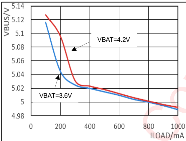
Figure 20 Load regulation for boost mode
