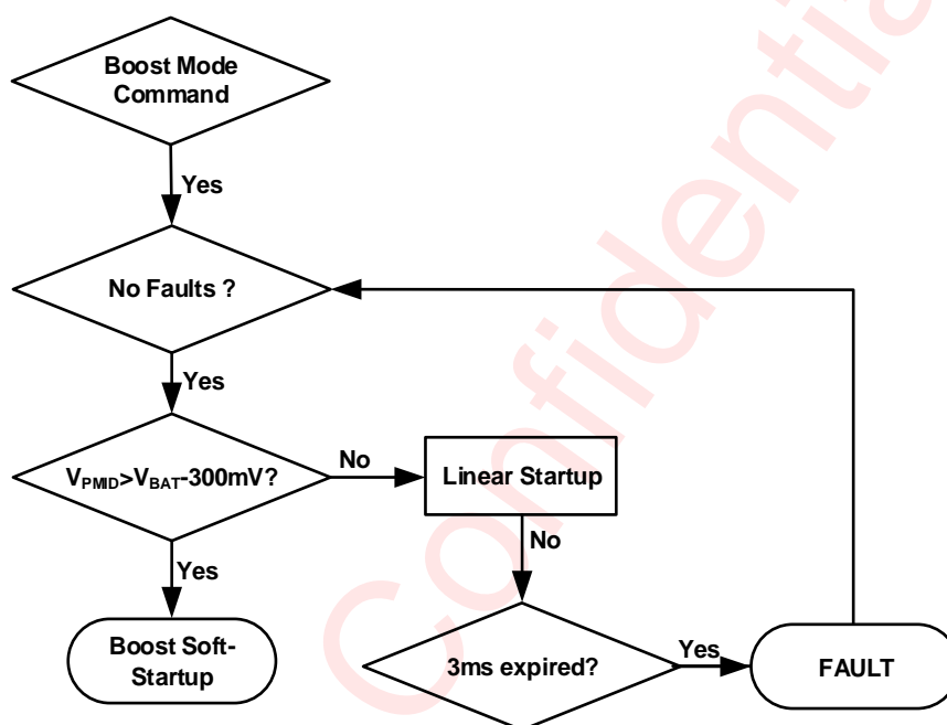
Figure 31 Boost Mode Start Scheme Flow Chart
