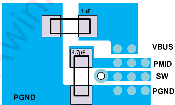
Figure 39 Input Capacitor Position and PCB Layout Example
