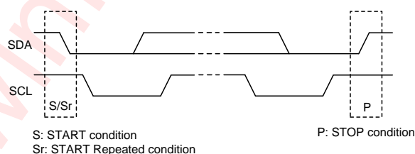
Figure 33 Start and Stop Conditions
