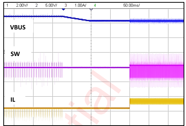
V_{BUS}=4.5V(CHG)/5.05V(BST) , V_{BAT}=3.5V Figure 25 Boost to charge mode transition
