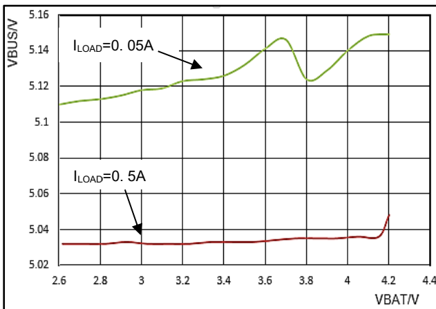
Figure 18 Line regulation for boost mode
