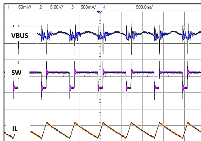
Figure 23 Boost FPWM waveform at light load
