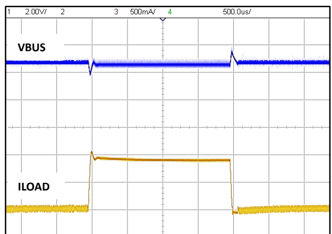
I_{LOAD}=5mA to 1A and to 5mA Figure 17 Load transient for boost mode
