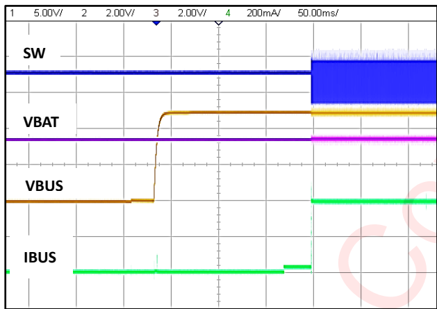
V_{BAT}=3.4V , OTG=1 Figure 14 Charge startup at VBUS plug-in
