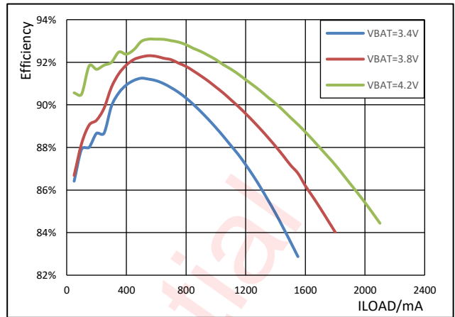
Figure 19 Efficiency for boost mode
