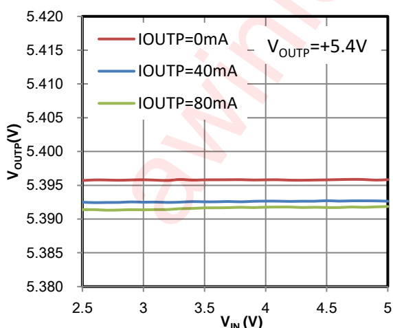
Figure 15 Line Regulation (80mA Mode)
