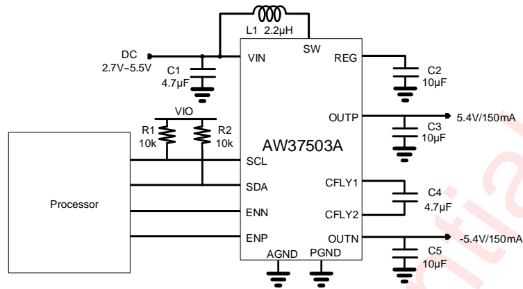
Figure 4 AW37503A Application circuit (150mA Mode)
