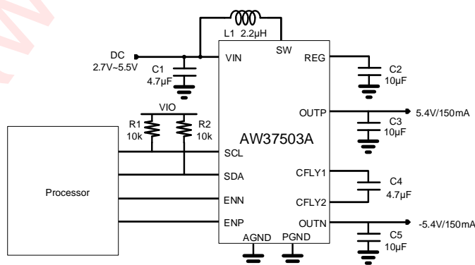
Figure 1 Typical Application Circuit of AW37503A
