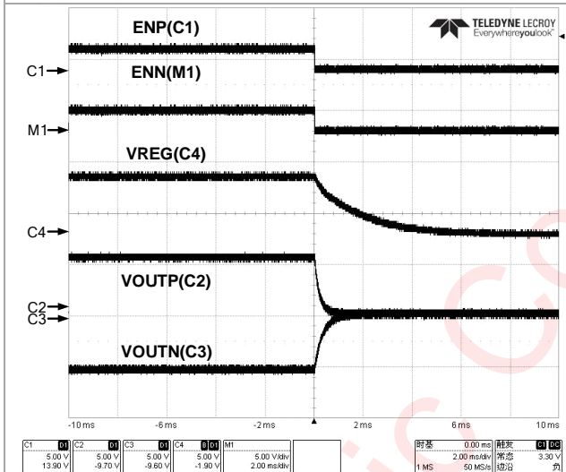
Figure 55 Power Down Sequencing (Simultaneous)
