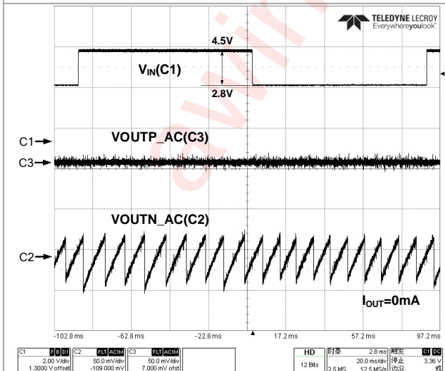
Figure 45 Line Transient (80mA Mode)
