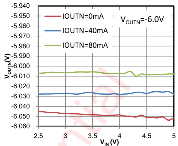
Figure 18 Line Regulation (80mA Mode)
