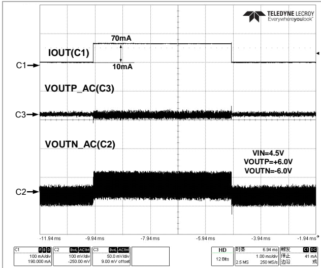
Figure 41 Load Transient(80mA Mode)
