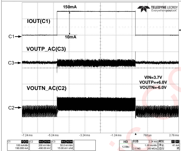
Figure 43 Load Transient(150mA Mode)
