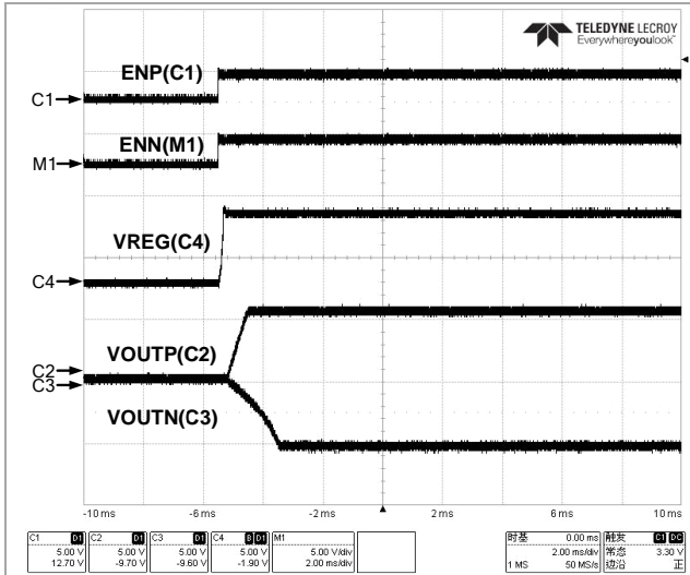
Figure 53 Power Up Sequencing (Simultaneous)
