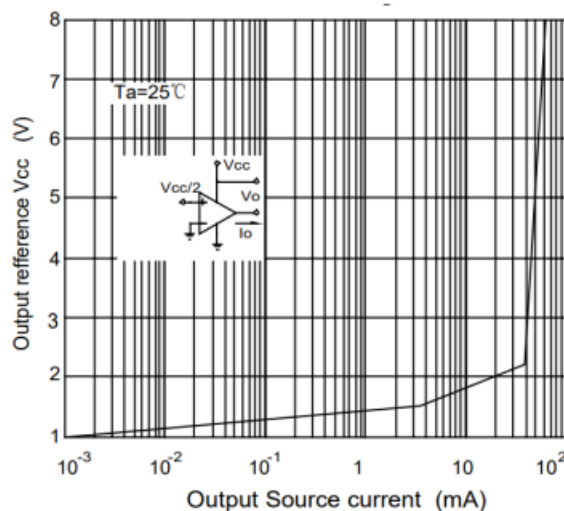
Fig.12 Current Limiting
