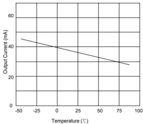
Fig.12 Current Limiting
