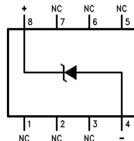
Figure 3. SOP8
