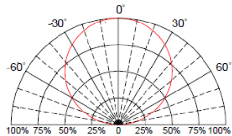
Fig.6 Directive Radiation
