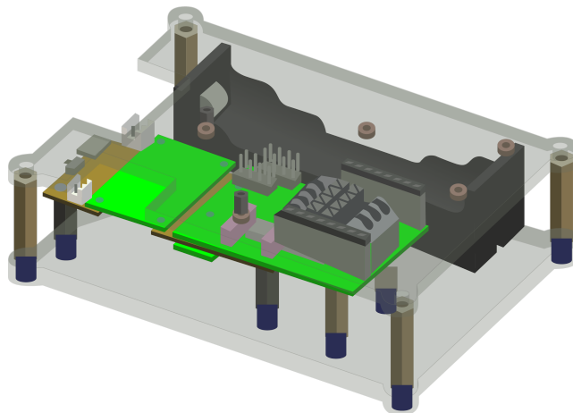
Figure 1: WisBlock RAKBox-B5 Enclosure Overview
