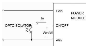
Isolated-Control Remote ON/OFF
