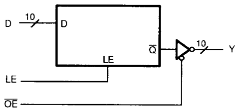
Am29841 10-Bit Latch
