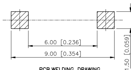
PCB.WELDING DRAWING
