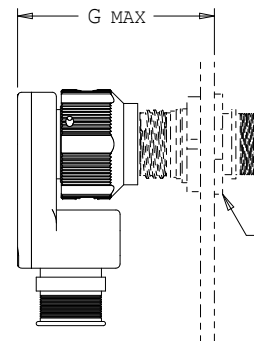
SQUARE FLANGE RECEPTACLE MATING SPACE REQUIREMENT
