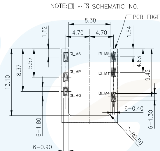
RECOMMENDED PADS LAYOUT <TOP VIEW> NOTE : TOLERANCE FOR PCB LAYOUT IS \pm 0.05
